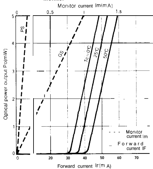
Fig. 67.2 Optical Power Output va. Forward Current and Monitor
