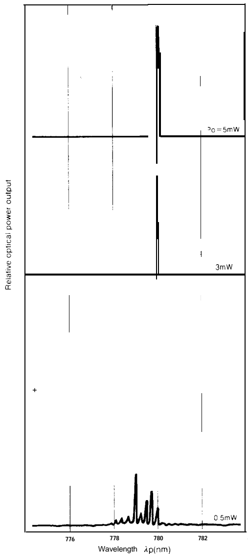
Fig. 67-5 Optical Power Output Dependence of Wavelength
