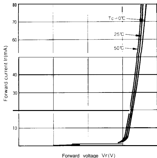
Fig. 67-1 Forward Current vs. Forward Voltage
