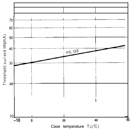
Fig. 67-3 Threshold Current vs. Temperature
